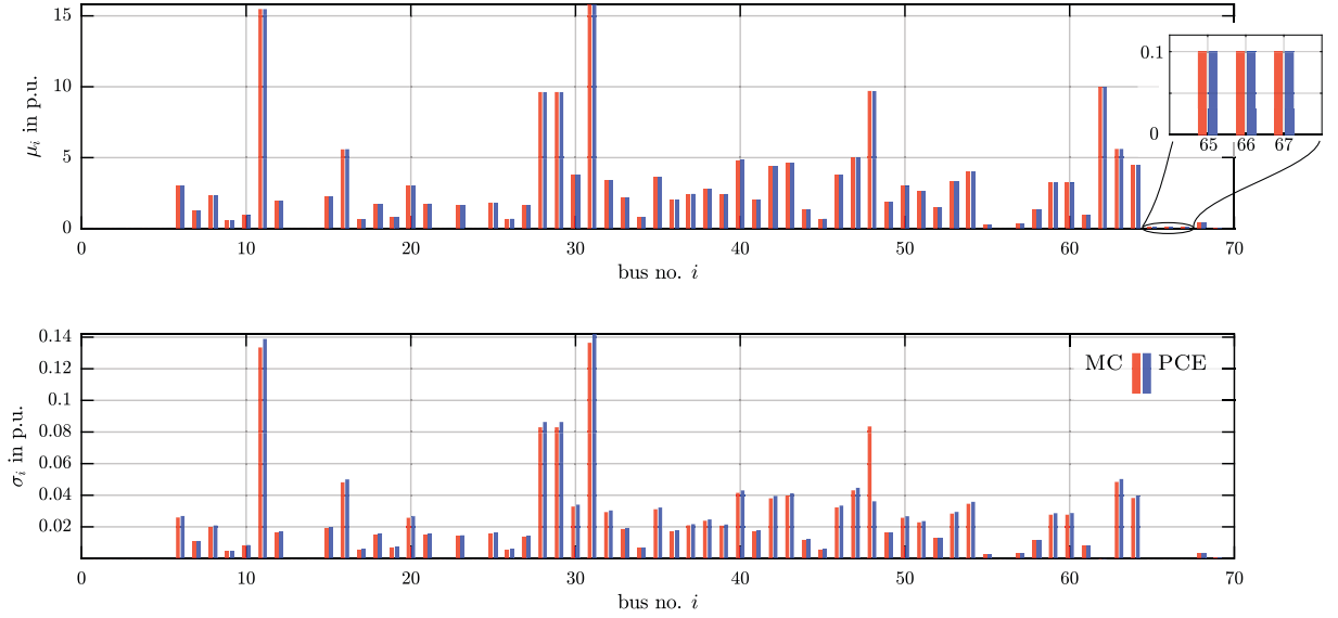
Fig. 1. Mean and standard deviation of generator buses i \in \mathcal{N}_g from MC and PCE solution.
